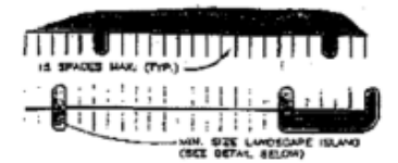
ACCEPTABLE LANDSCAPE ISLAND LAYOUT
