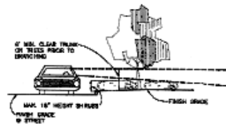
LANDSCAPE MATERIAL IN SIGHT DISTANCE AREA
