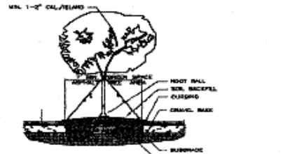
PROPER INSTALLATION TREE PLANTING FOR PARKING LOT ISLAND NOT TO SCALE
